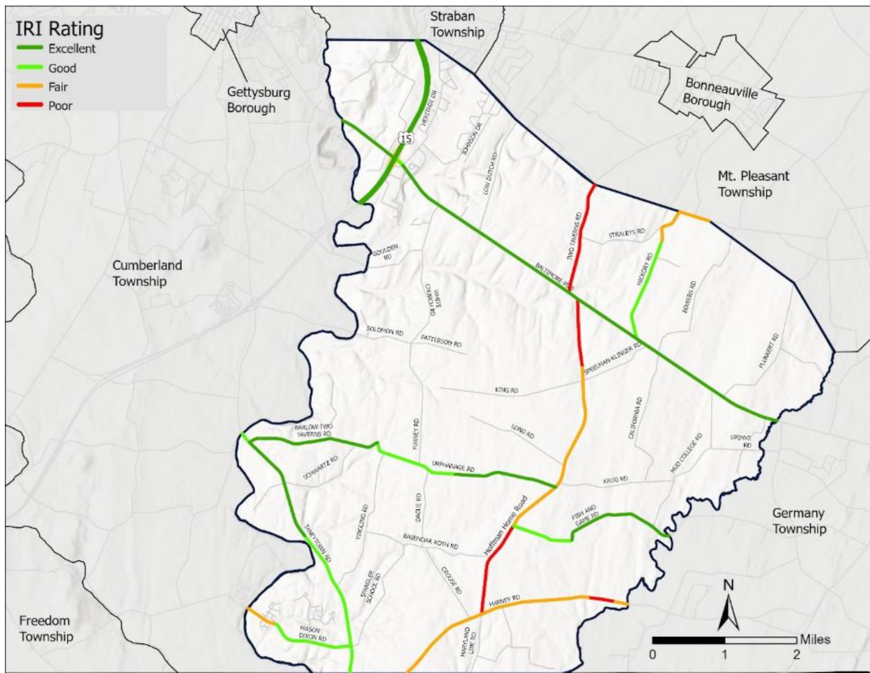
Figure 9: IRI Rating
